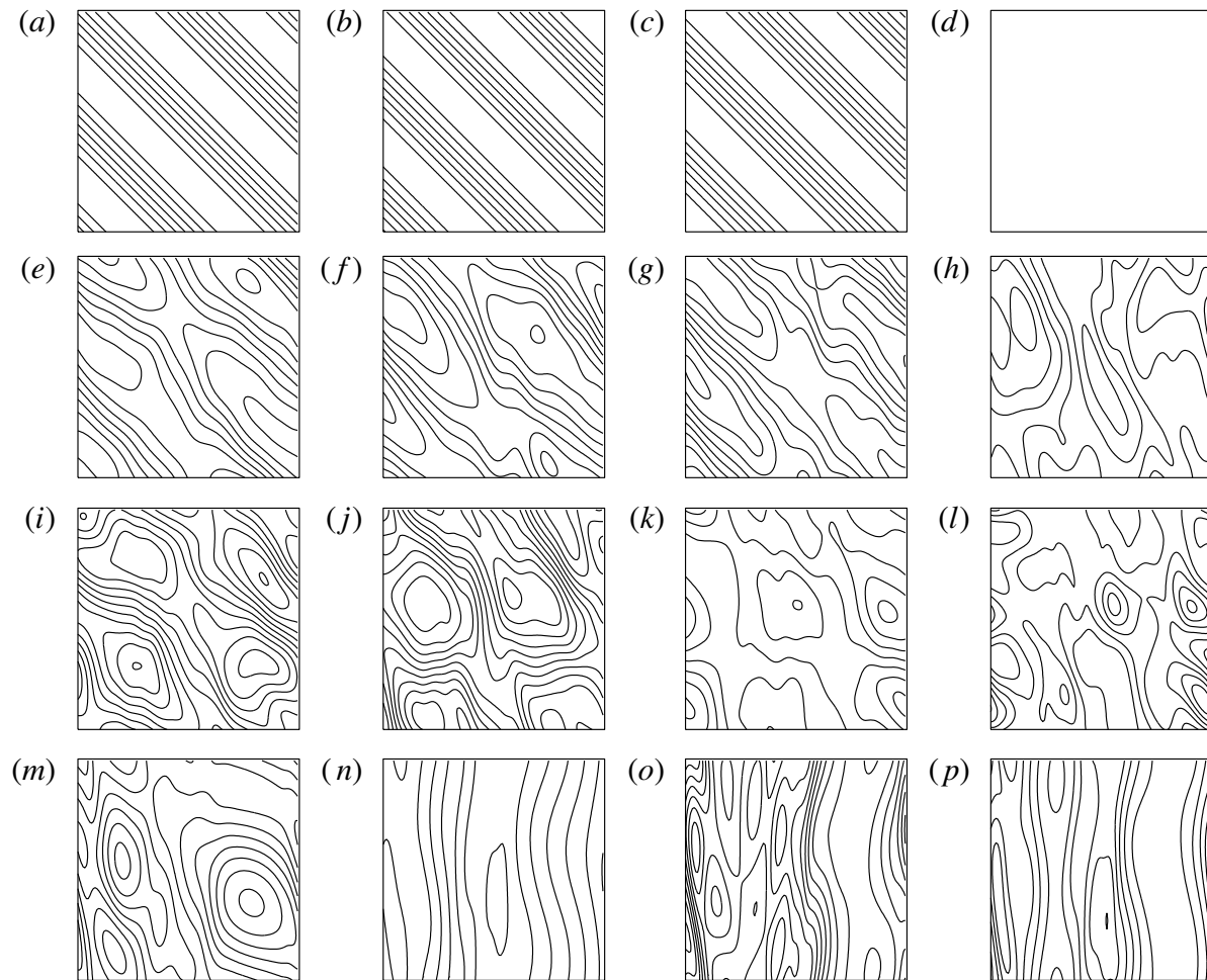
FIGURE 5. The contours of velocity in the x - z plane at y=0 for the snapshot at time = 10 000. In each row the panels from left to right are contours of respectively u_1 ( a, e, i, m ), u_2 ( b, f, j, n ), u_3 ( c, g, k, o ) and kinetic energy ( d, h, l, p ). At the resonant frequency, \omega = -2/\sqrt{3} corresponding to figure 4(a). ( a - d ) Linear response with a = 1 \times 10^{-3} (kinetic energy is constant). ( e - h ) Nonlinear response with a = 1 \times 10^{-3} . ( i - l ) Nonlinear response with a = 2 \times 10^{-3} . ( m - p ) Nonlinear response with a = 3 \times 10^{-3} .
