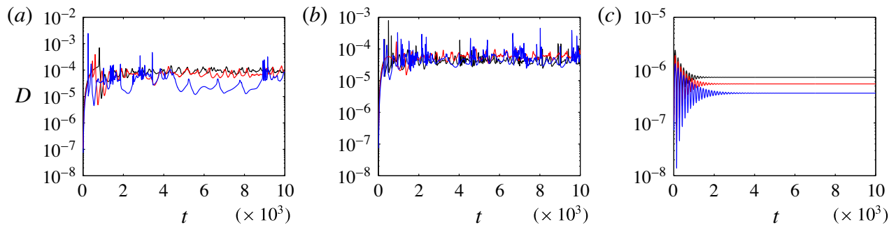
FIGURE 7. (Colour online) The investigation of the Ekman number in the nonlinear regime. The dissipation D versus time with a = 1 \times 10^{-3} and k_x = k_y = k_z = 1 . (a) The resonant frequency \omega = -2/\sqrt{3} . (b) Frequency \omega = -1.16 near the resonant frequency. (c) Frequency \omega = -1.2 far away from the resonant frequency. Black, red and blue lines (from top downwards in (c)) denote the nonlinear regime at respectively E = 1 \times 10^{-3} , 7.5 \times 10^{-4} and 5 \times 10^{-4} .
