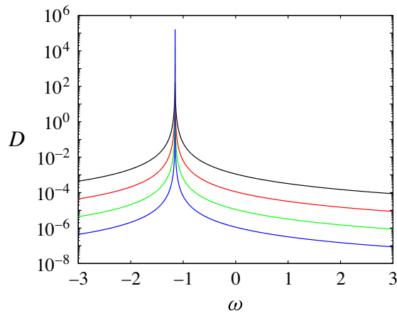
FIGURE 1. (Colour online) The investigation of the force frequency in the linear regime. The dissipation D versus the force frequency \omega , for a = 1 and k_x = k_y = k_z = 1 . Black, red, green and blue lines (from top downwards) denote, respectively, E = 10^{-3} , 10^{-4} , 10^{-5} and 10^{-6} .
