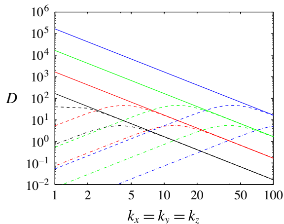
FIGURE 2. (Colour online) The investigation of the force wavenumber in the linear regime. The dissipation D versus the force wavenumber k_x = k_y = k_z , for a = 1 . Black, red, green and blue lines (from bottom upwards for the straight lines) denote, respectively, E = 10^{-3} , 10^{-4} , 10^{-5} and 10^{-6} . Solid lines denote the resonant frequency \omega = -2/\sqrt{3} , dashed lines \omega = -1.16 near the resonant frequency, and dash-dotted lines \omega = -1.2 far away from the resonant frequency.
