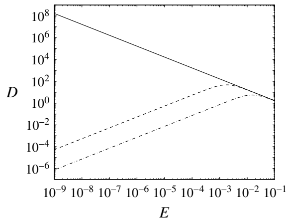
FIGURE 3. The investigation of the Ekman number in the linear regime. The dissipation D versus the Ekman number E , for a=1 and k_x=k_y=k_z=1 . Solid line denotes \omega = -2/\sqrt{3} , dashed line \omega = -1.16 near the resonant frequency, and dash-dotted line \omega = -1.2 far away from the resonant frequency.
