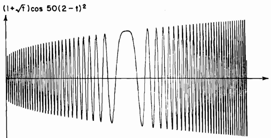
Figure 3-5. A function with a stationary point.
