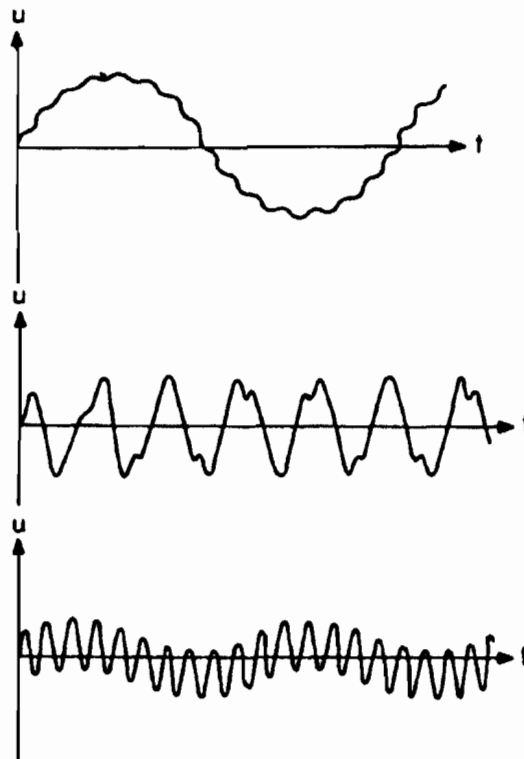
Figure 11-2. Bounded solutions of the Mathieu equation.
