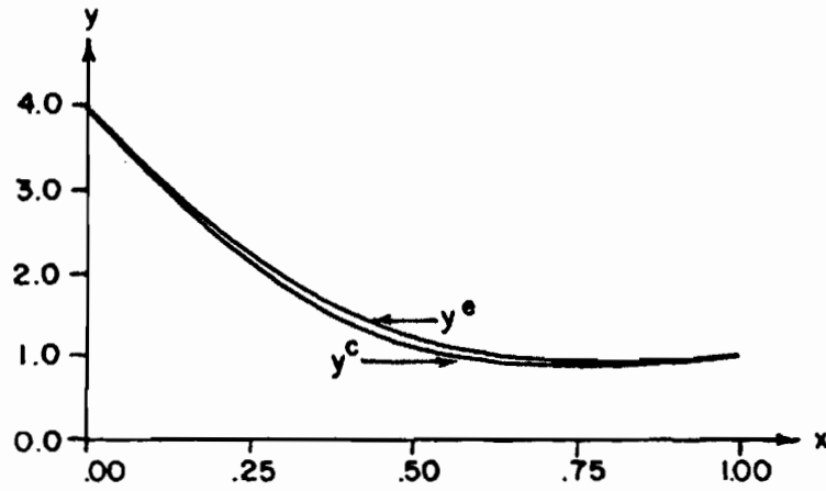
Figure 12-10. Comparison of the composite expansion y^c with the exact solution y^e obtained by numerically integrating (12.131) and (12.102) for \epsilon = 0.2 , \alpha = 4.0 , \beta = 1.0 .
