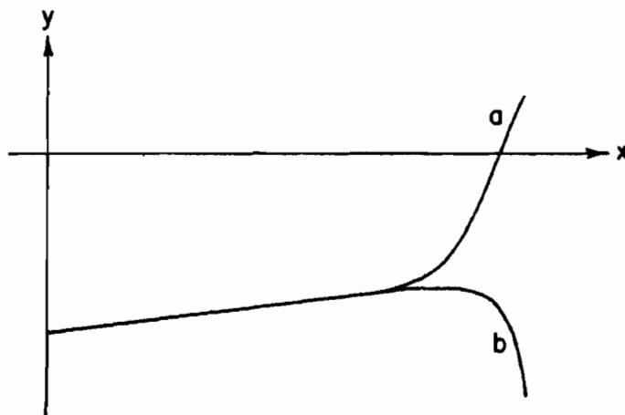
Figure 12-16. Behavior of the composite solution when the boundary layer is at x = 1 for \epsilon = 0.1 , \alpha = -3 and: (a) R = 1 , (b) R = -4
