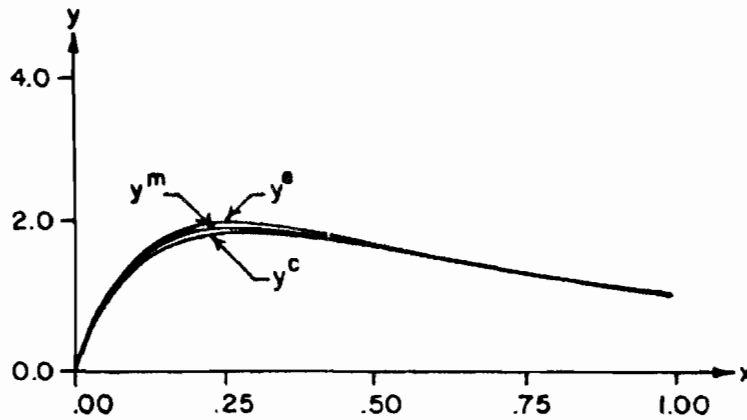
Figure 12-8. Comparison of the method-of-multiple-scales solution y^m with the composite expansion y^c and the exact solution y^e for \epsilon = 0.1 , \beta = 1.0 , and \alpha = 0.0 .
