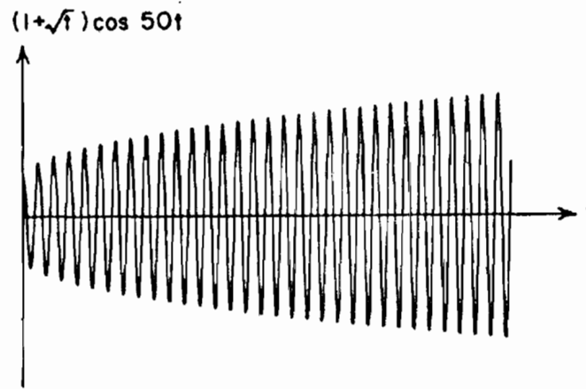
Figure 3-4. A function with rapid oscillations.
