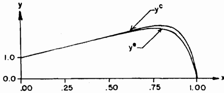
Figure 12-9. Comparison of composite expansion y^c with the exact solution y^e obtained by numerically integrating (12.103) and (12.102) for \epsilon = 0.2 , \alpha = 1.0 , and \beta = 0.0 .
