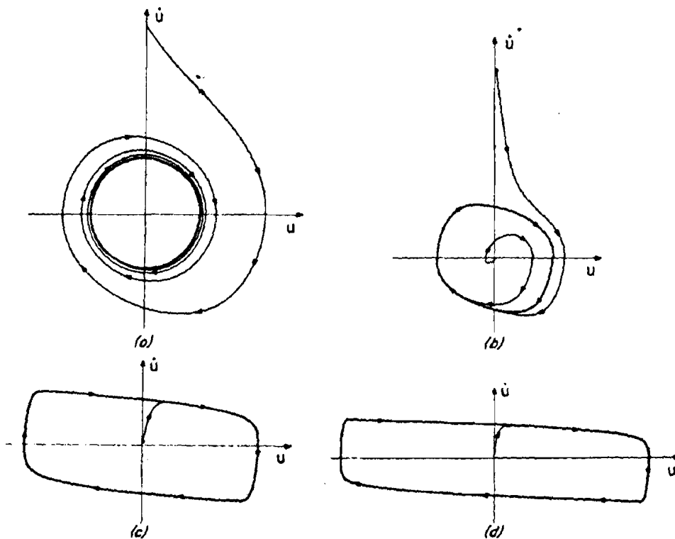
Figure 6-2. Phase planes for Rayleigh's equation: (a) \epsilon = 0.01 ; (b) \epsilon = 0.1 ; (c) \epsilon = 1 ; (d) \epsilon = 10.0 .
