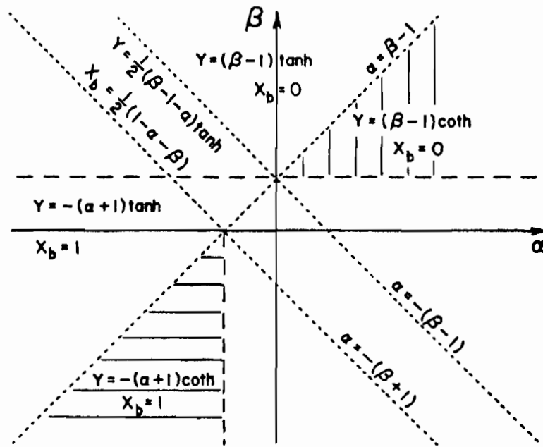
Figure 12-18. A diagram that summarizes the location of the boundary layer in the \beta\alpha -plane.
