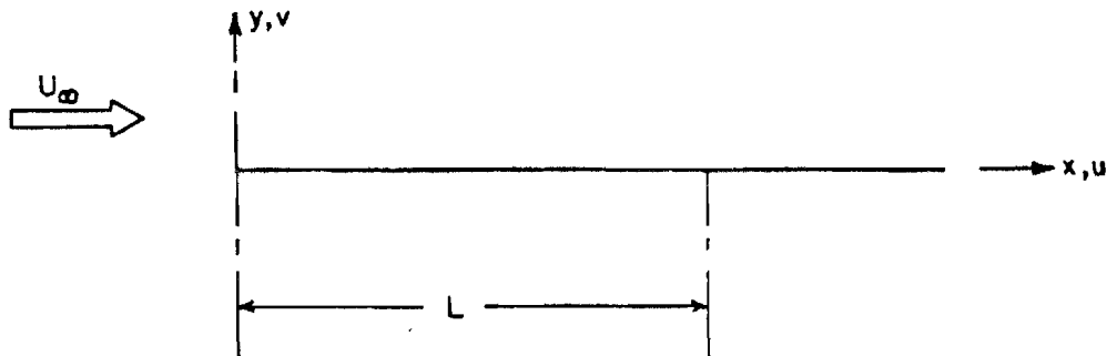
Figure 1-3. Flow past a flat plate.
