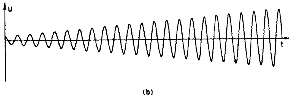
Figure 6-1. Comparison of straightforward expansion (a) with exact solution (b) for u(0) = 0.5 , \dot{u}(0) \approx 0 , and \epsilon = 0.1 .
