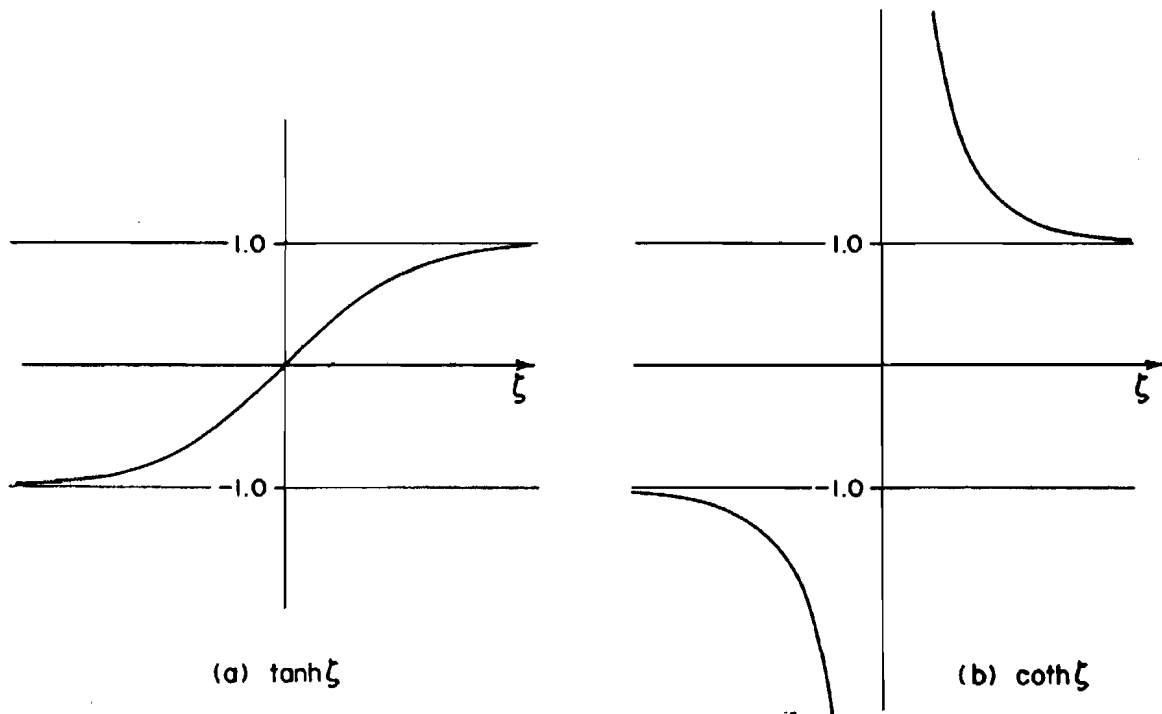
Figure 12-14. Behavior of \tanh\zeta and \coth\zeta .
