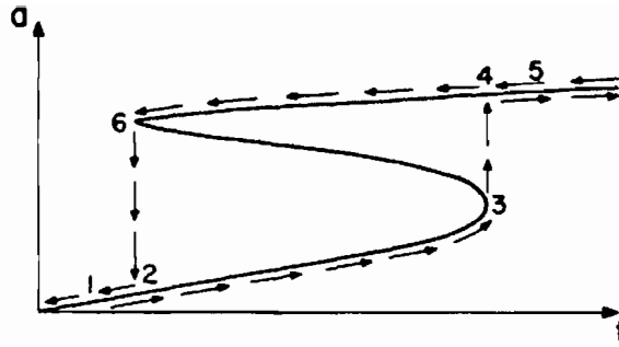
Figure 9-8. Jump phenomena for primary resonance of the Duffing equation.
