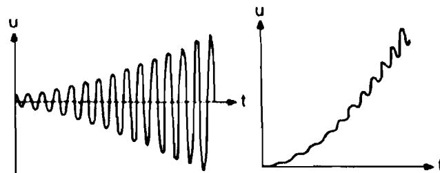
Figure 11-1. Unbounded solutions of the Mathieu equation.
