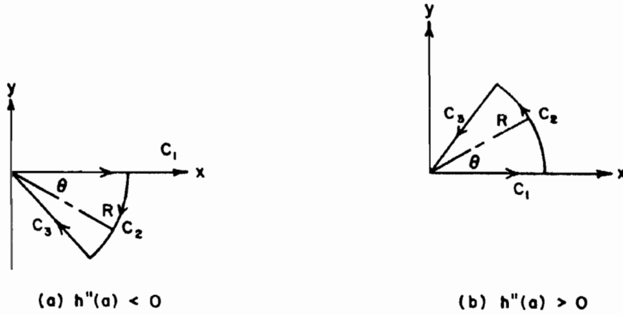
Figure 3-6. Deformation of the contour of integration.
