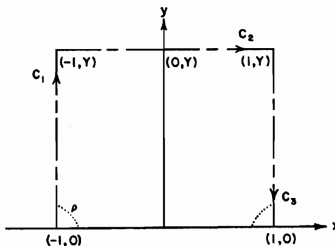
Figure 3-10. Contour deformation for (3.219).
