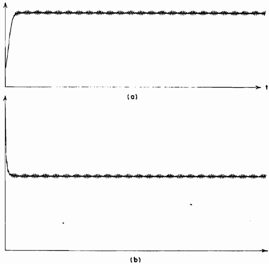
Figure 6-4. Comparison of solutions of the variational equations (6.68) and (6.69) with those of the averaged equation (6.70) for \epsilon = 0.3 : (a) a(0) = 0.5 , \beta(0) = 0 ; (b) a(0) = 4.0 , \beta(0) = 0 .
