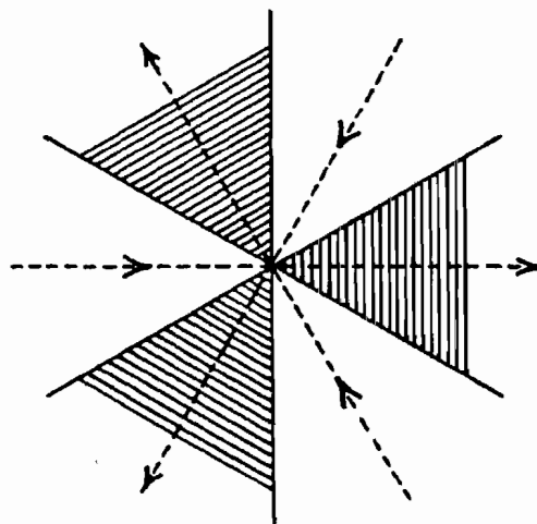
Figure 3-9. Topography of the surface \phi = \operatorname{Re} h(z) near a saddle point of order 3 when \chi = 0 . The valleys are shaded, the steepest curves dotted, the solid lines are the level curves, and the arrows indicate the direction in which \phi decreases.
