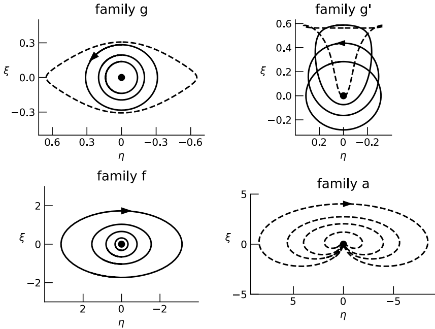
Figure 3.11: Examples of periodic orbits in Hill's problem. Each orbit is shown by a solid line if stable, and by a dashed line if unstable. The origin is marked by a black circle. Additional orbits in family g' can be derived by reflection in the line \xi = 0 . Orbits in family c can be derived from orbits in family a by the same reflection. Note that the horizontal or \eta -axis increases from right to left, as in Figures 3.9 and 3.13. The values of the Jacobi–Hill constant E_H for each family are: family g , -1.5, -2.25, -3, -4 ; family g' , -2.25, -2.2, -2.13571, -2 ; family f , 1.5, 0.5, 0, -1 ; family a , 4.5, 2, 1, 0 . The orbits in families g and g' with E_H = -2.25 and E_H = -2.13571 respectively are the last stable members of each family.
