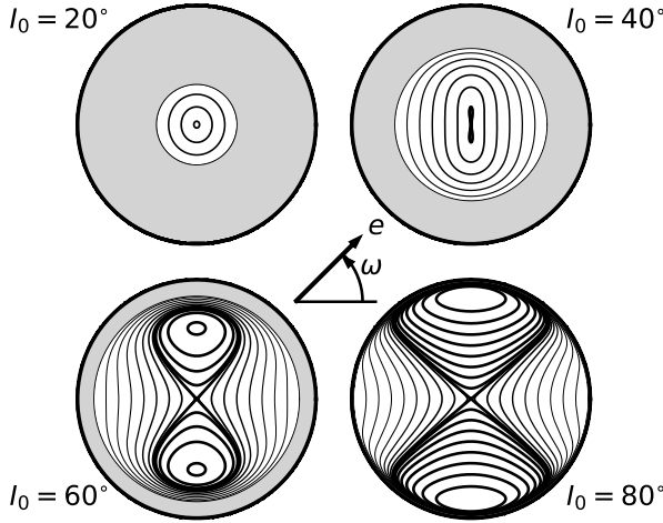
Figure 5.4: Contours of the ZLK function C_{\text{ZLK}}(e, \omega) (eq. 5.97), with the eccentricity e and argument of periaapsis \omega plotted as polar coordinates. Shaded regions have e > \sin I_0 and are unphysical. Plots are shown for four values of I_0 , the inclination of a circular orbit. Prograde circular orbits are unstable for I_0 > I_{\text{ZLK}} = 39.23^\circ . Heavy contours have C_{\text{ZLK}}(e, \omega) \geq 0 . Compare Figure 9.5.
