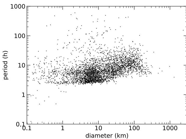
Figure 8.1: The distribution of spin periods, in hours, of \simeq 3\,700 asteroids as a function of diameter. Data from Warner et al. (2019), restricted to asteroids with rotation period quality code U3 (highest).
