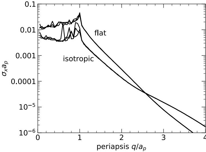
Figure 9.3: Root-mean-square change in x = 1/a for an initially parabolic orbit during a single periastris passage through a planetary system. The system contains a single planet on a circular orbit with semimajor axis a_p , having mass 0.001 times the stellar mass. Each curve is determined from 10^4 incoming orbits with random values of the longitude of node and periastris. Three Monte-Carlo realizations are shown for each curve to indicate the uncertainties. The inclinations of the parabolic orbits are chosen from either a Rayleigh distribution with mean inclination \langle I \rangle = 10^\circ (labeled “flat”) or a uniform distribution in \cos I (labeled “isotropic”).
