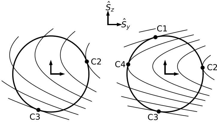
Figure 7.4: The state of Colombo's top is defined by the components (\hat{S}_x, \hat{S}_y, \hat{S}_z) of the unit spin vector in the non-inertial frame, where \hat{z} is parallel to the satellite's orbital angular momentum and \hat{x} points to the ascending node of the satellite orbit on the orbit of its host planet. The figure shows the \hat{S}_x = 0 plane for p = q = 0.5 (left panel) and p = q = 0.2 (right panel). The unit spin vector is restricted to the circle \hat{S}_y^2 + \hat{S}_z^2 = 1 , and the parabolas opening to the right are the contours of the Hamiltonian (7.67). The Cassini states, labeled C1, C2, C3, C4, are located where the contours of the Hamiltonian are tangent to the unit circle.
